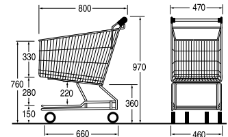
Ref. 7 769 02 03 Nesting distance: 230 mm
