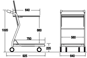
Ref. 4 454 08 03 Nesting : 242 mm
