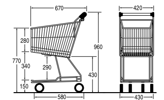
Ref. 7 768 62 03 Nesting distance: 175 mm
