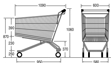
Ref. 7 722 90 03 Nesting distance: 230 mm
