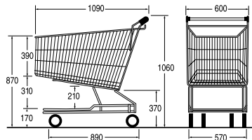
Ref. 7 767 90 03 Nesting distance: 246 mm
