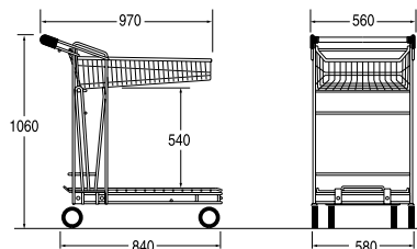
Ref. 4 455 03 03 Nesting distance: 270 mm
