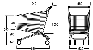
Ref. 7 781 32 03 Nesting distance: 222 mm
