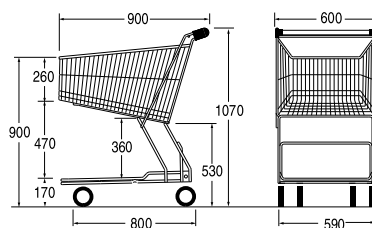
Ref.7 727 25 03 Nesting distance: 190 mm
