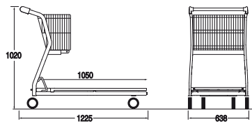
Ref. 4 454 11 03 Nesting distance: 352 mm Permitted load: 250 kg
