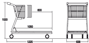
Ref. 4 454 11 03 Nesting distance: 352 mm
