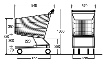
Ref. 7 767 50 03 Nesting distance: 259 mm
