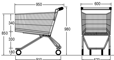
Ref. 7 721 20 03 Nesting distance: 220 mm
