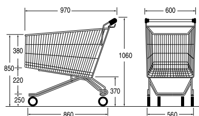
Ref. 7 722 80 03 Nesting distance: 230 mm
