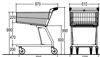
Ref. 7 788 80 03 Nesting distance: 225 mm
