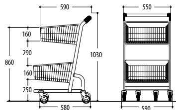
Ref. 7 788 12 03 Nesting distance: 190 mm
