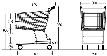
Ref. 7 795 00 03 Nesting distance: 266 mm
