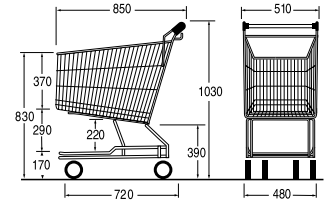
Ref. 7 767 25 03 Nesting distance: 231 mm
