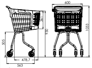
Ref. 7 784 01 03 Nesting distance: 150 mm Registered design
