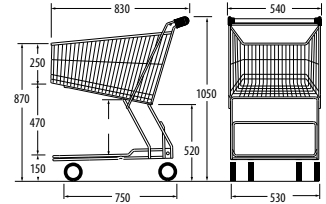
Ref. 7 727 00 03 Nesting distance: 145 mm
