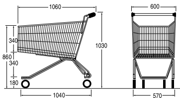
Ref. 7 735 00 03 Nesting distance: 220 mm
