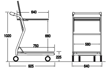
Ref. 4 454 08 03 Nesting distance: 242 mm Permitted load: 250 kg
