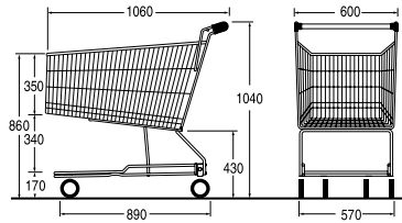
Ref. 7 734 60 03 Nesting distance: 220 mm
