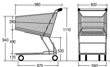
Ref.7 727 50 03 Nesting distance: 210 mm
