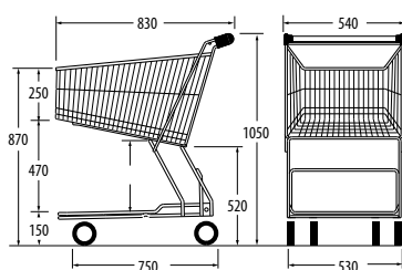
Ref.7 729 00 03 Nesting distance: 145 mm
