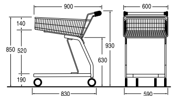
Ref. 7 788 51 03 Nesting distance: 250 mm
