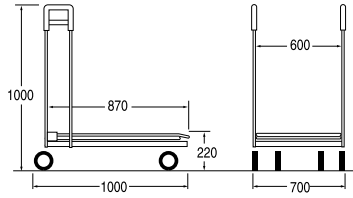
Ref. 4 499 75 03 Nesting distance: 330 mm Permitted load: 250 kg
