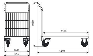
Ref. 4 430 10 03 Permitted load: 400 kg
