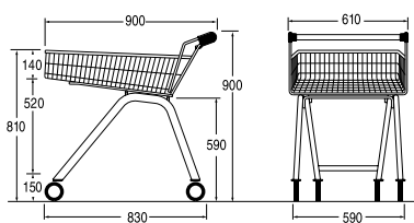
Ref. 7 788 70 03 Nesting distance: 250 mm
