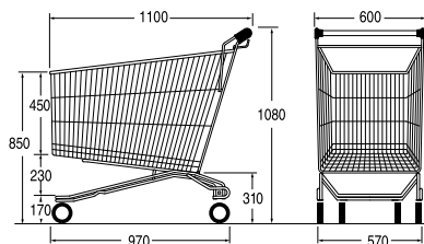
Ref. 7 770 10 03 Nesting distance: 230 mm
