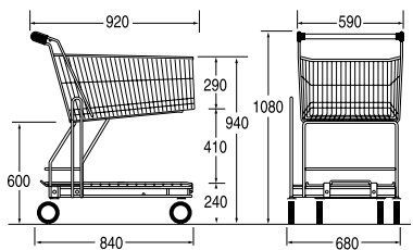
Ref. 4 455 00 03 Nesting distance: 270 mm
