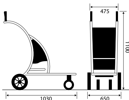
Ref. 7 713 80 97 10 nested trolleys: 3350 mm
