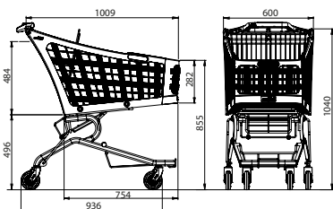
Ref. 7 786 03 03 Nesting distance: 270 mm
