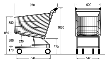
Ref. 7 767 80 03 Nesting distance: 249 mm
