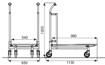
Ref. 4 459 40 03 Nesting distance: 275 mm Permitted load: 300 kg
