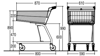
Ref. 7 788 80 03 Nesting distance: 225 mm
