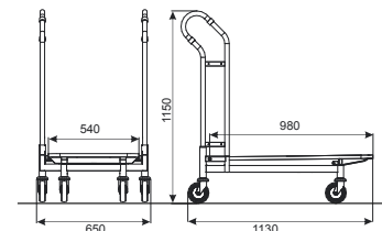
Ref. 4 459 45 03 Nesting distance: 275 mm Permitted load: 300 kg
