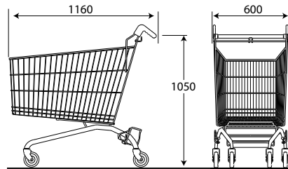
Ref. 7 780 01 03 Nesting distance: 240 mm
