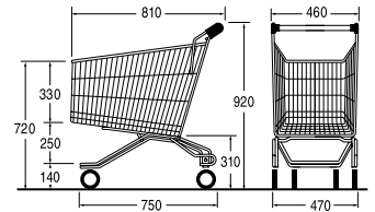
Ref. 7 777 30 03 Nesting distance: 225 mm
