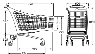
Ref. 7 786 01 03 Nesting distance: 285 mm
