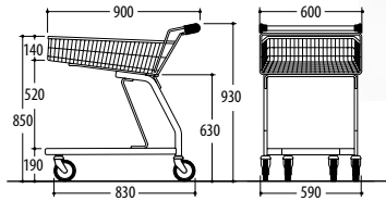
Ref. 7 788 51 03 Nesting distance: 250 mm
