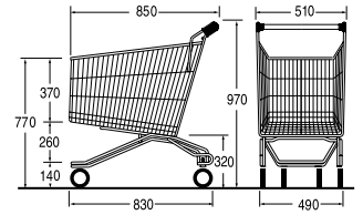
Ref. 7 778 32 03 Nesting distance: 215 mm
