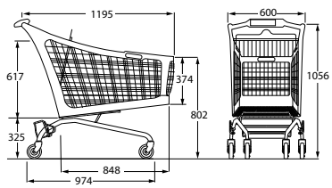
Ref. 7 786 02 03 Nesting distance: 285 mm
