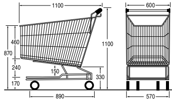
Ref. 7 767 40 03 Nesting distance: 250 mm
