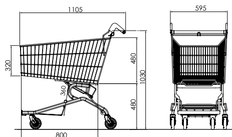
Ref. 7 780 03 03 Nesting distance: 270 mm
