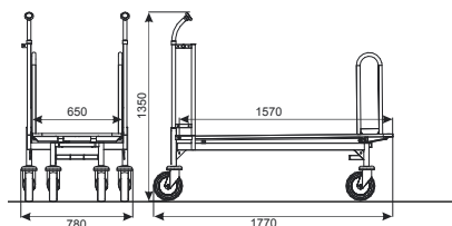
Ref. 4 459 60 03 Nesting distance: 445 mm Permitted load: 500 kg
