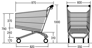
Ref. 7 797 32 03 Nesting distance: 250 mm
