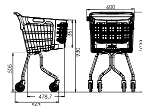
Ref. 7 784 01 03 Nesting distance: 150 mm Registered design
