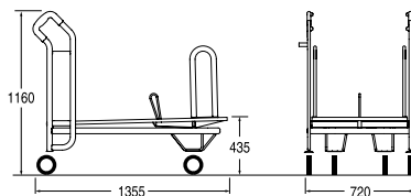
Ref. 4 459 50 03 Nesting distance: 325 mm Permitted load: 500 kg
