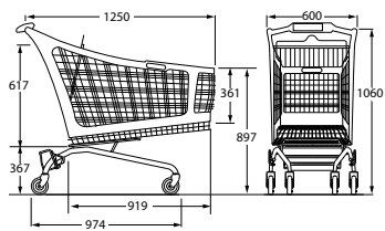
Ref. 7 786 04 03 Nesting distance: 295 mm
