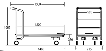
Ref. 4 459 70 03 Nesting distance: 340 mm Permitted load: 350 kg
